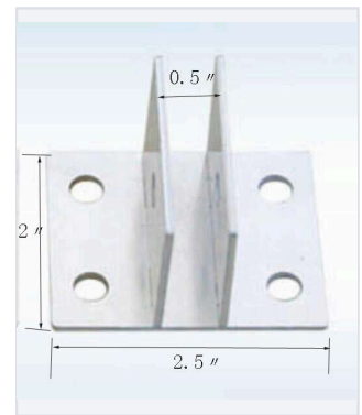
LKG-2 Mounting bracket · 2.5"
