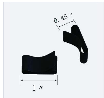
HQZ-1 24 Sign corner clip · 1" × 0.45"
