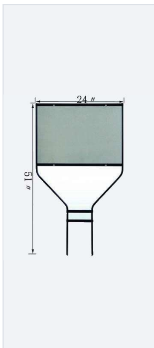
09 DZJ2451 Ground stake frame · 24" × 51"
