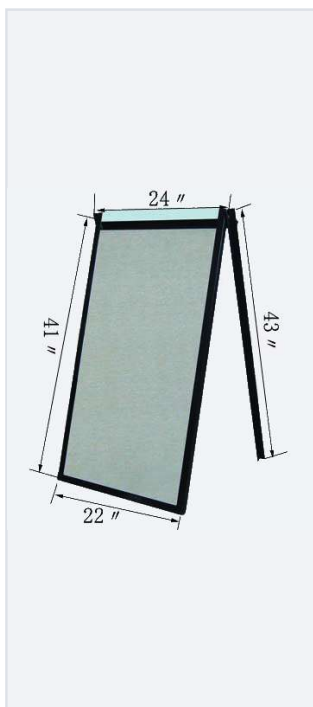
14 SZJ-A Angled stake frame · 24" × 41"
