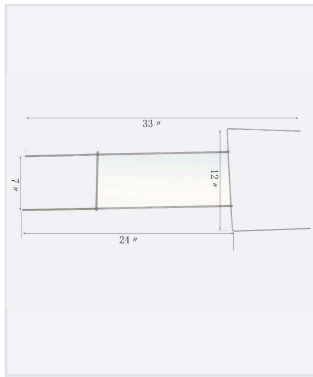
TS-A Wire step stake
