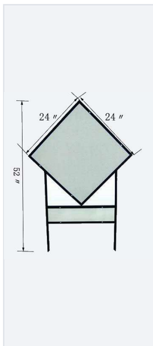
15 DZJ2452 Diamond stake frame · 24" × 24" panel
