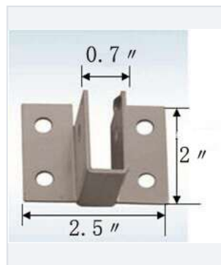
LKG-4 Mounting bracket · 2" × 2.5"
