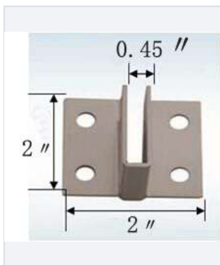
LKG-3 Mounting bracket · 2" × 2"
