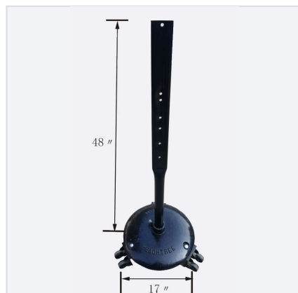
DTG-1 23 Post with cast base · 48" × 17"
